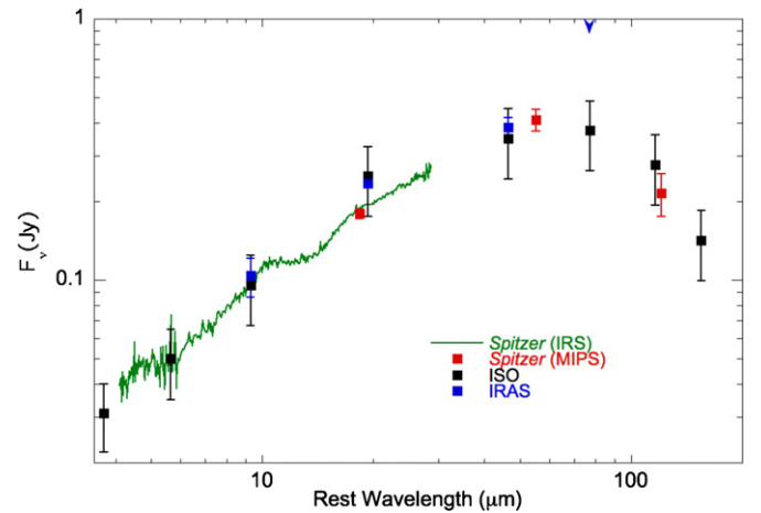
Figure 6. Spectral energy distribution of the PG 1700+518 system. Plotted data are from IRAS , ISO , and Spitzer Space Telescope . The IRS spectrum is from Shi et al. (2007), and the MIPS photometry is from D. Hines 2009, private communication.
