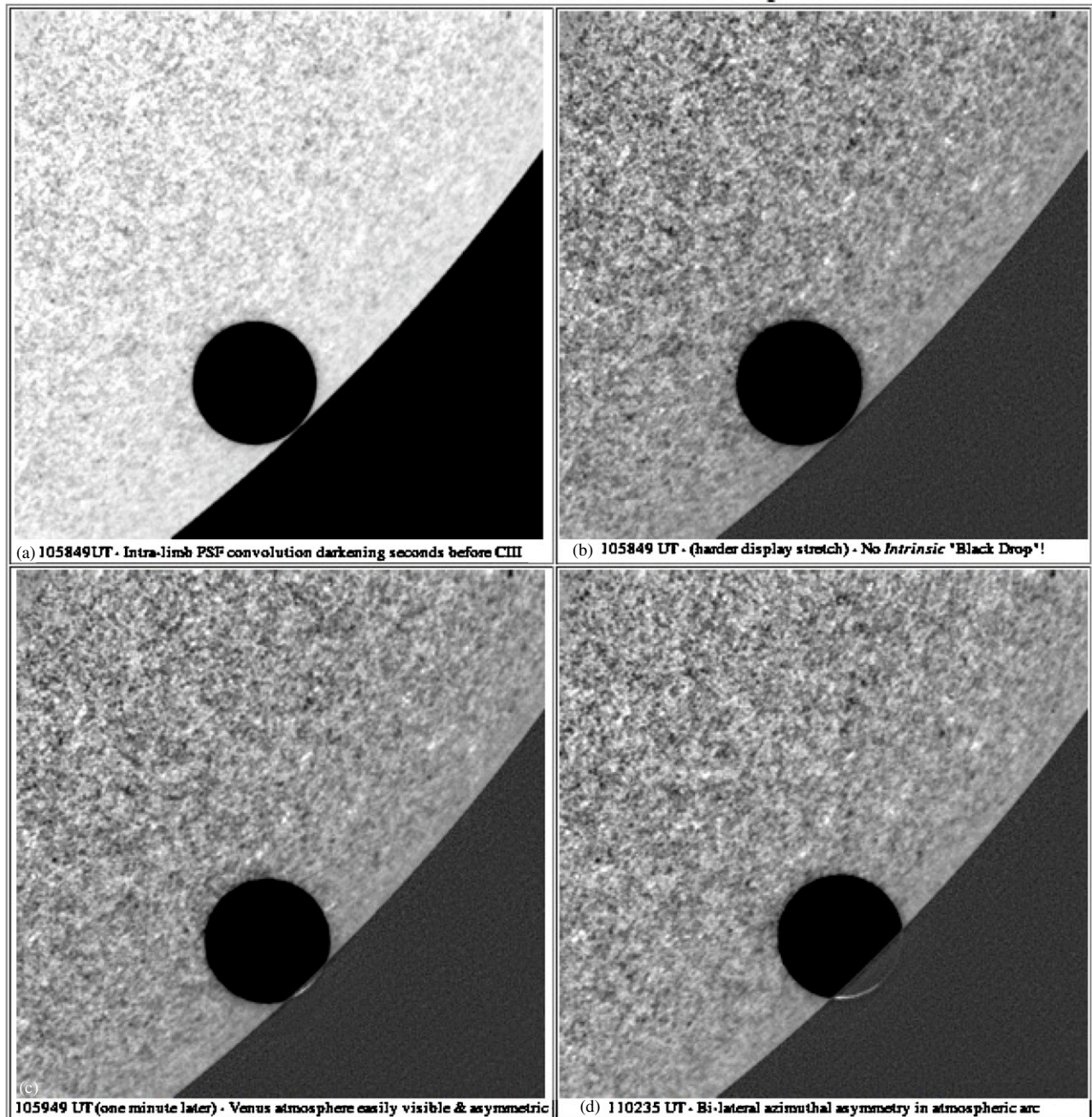
Figure 4. Egress. (a) Third contact (10:58:49 UT). (b) As in Figure 3(c), a minor black-drop of instrumental + limb-darkening origin is seen in contrast-enhanced frame (b) (same data as frame (a)). (c) First visibility of Venus’s atmosphere after the contact (10:59:49 UT). (d) The brightness asymmetry along the Cytherean atmospheric arc in, and flanking, the southern polar region after third contact (11:02:35 UT) is similar to what was reported by Russell for the 1874 transit (see Figure 1; Link 1969; Tanga 2004). The observed aureole results from the refraction of solar photospheric emission by the limb upper atmosphere of Venus. The asymmetry results from latitudinal differences in atmospheric refractive properties (see Section 3.2).
