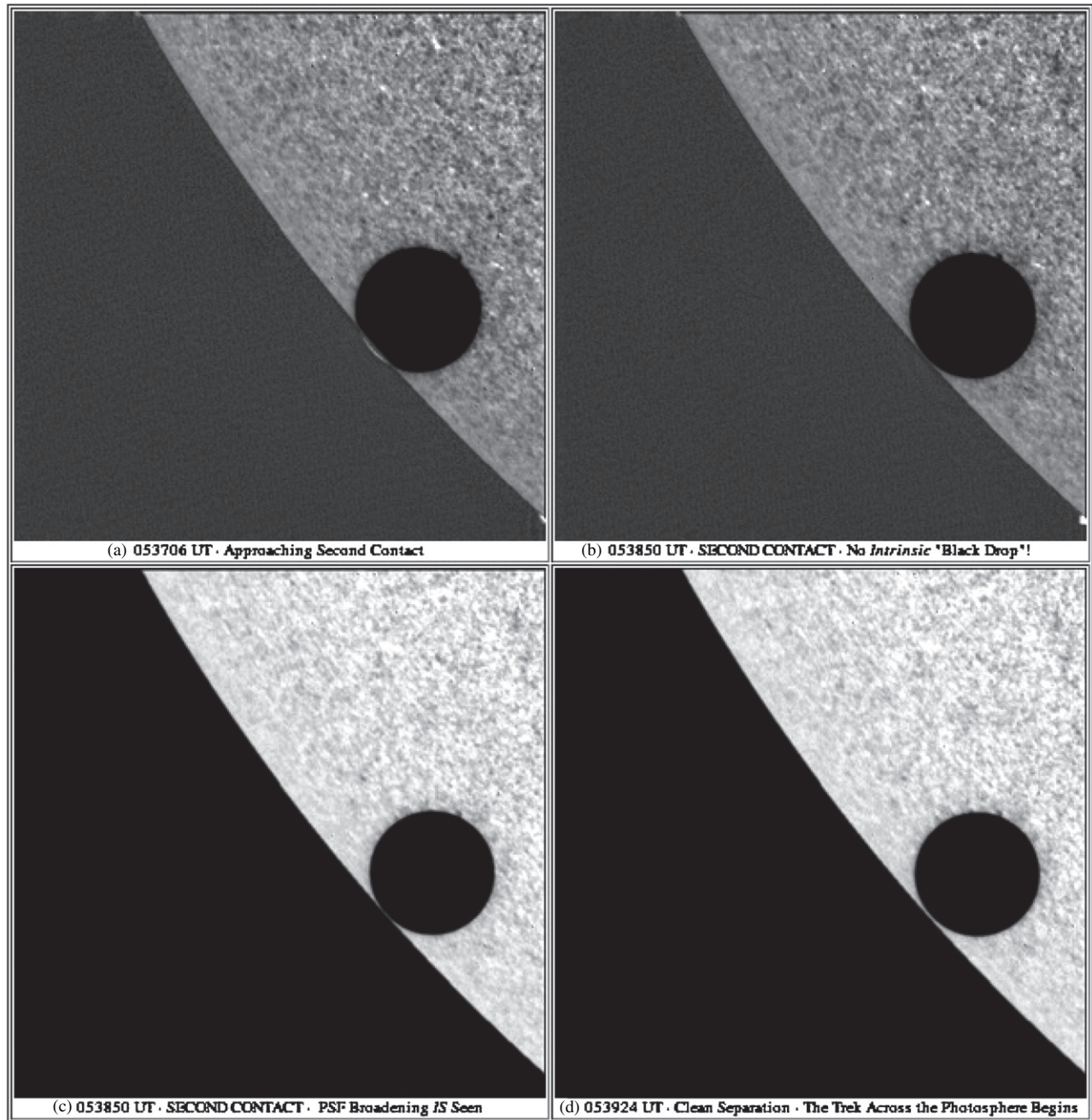
Figure 3. Ingress sequence at second contact. (a) The Cytherean atmosphere remains visible just before second contact (05:37:06 UT) while (b) no intrinsic black drop is apparent. (c) Enhancement of frame (b) shows a minor artifact black-drop effect (from the convolution of the telescope + instrument point-spread function with the solar limb-darkened photosphere backlighting Venus near the point of limb tangency). (d) Any apparent instrumental/limb-darkening black drop has disappeared by the time the tangent point of second contact is 850 mas from the planet's limb (05:39:24 UT). Image processing of frames (c) and (d) has purposefully intensified the section of the image outside the solar limb with respect to the solar photosphere; see the text for details.
