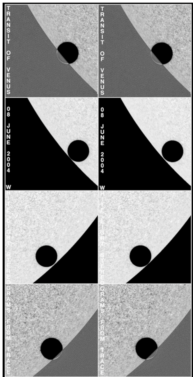
Figure 6. Stereograms, with pairs of images taken over short intervals of time. The stereo effect can be seen by most people by simply letting the eyes relax. The 3D effect is more profound in the high-resolution images that are available in the online edition. They can be viewed from a larger distance, which is more relaxing for the eyes.
