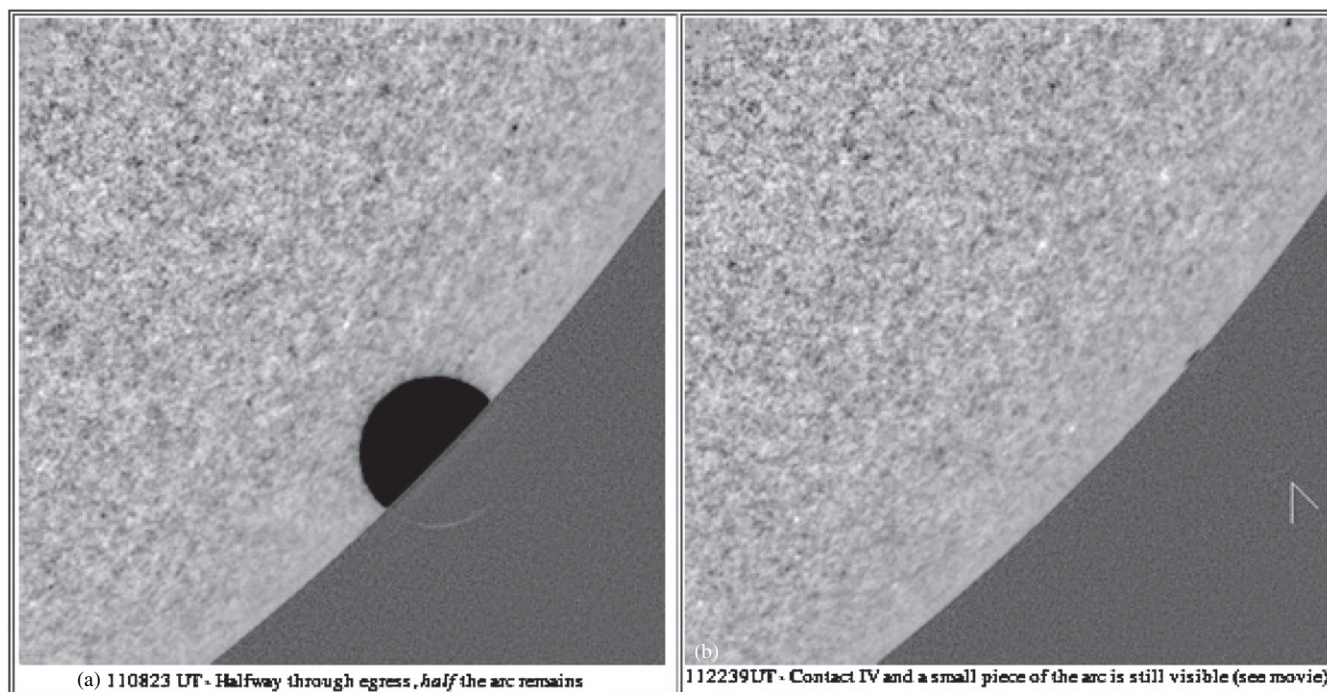
Figure 5. Egress. (a) At geometrical mid-egress (11:08:23 UT), about half of the illuminated arc of Venus’s atmosphere remains visible. With the gradual disappearance of Venus’s illuminated atmosphere, refracted solar radiation at diminished intensity asymmetrically persists along the atmospheric arc extending \sim 30^\circ in latitude from the Cytherean south pole. This atmosphere region is dynamically enclosed in a bulge of cold air (polar collar) and where the Venus cloud tops are lower by 7–10 km than at lower latitudes (see Section 4). (b) Seconds before fourth contact (11:22:39 UT), with only a tiny bit of Venus’s dark disk silhouetted against the solar photosphere at the point of limb tangency, a small, faint sliver of the atmospheric arc near the south pole remains visible (location marked with an arrow).
