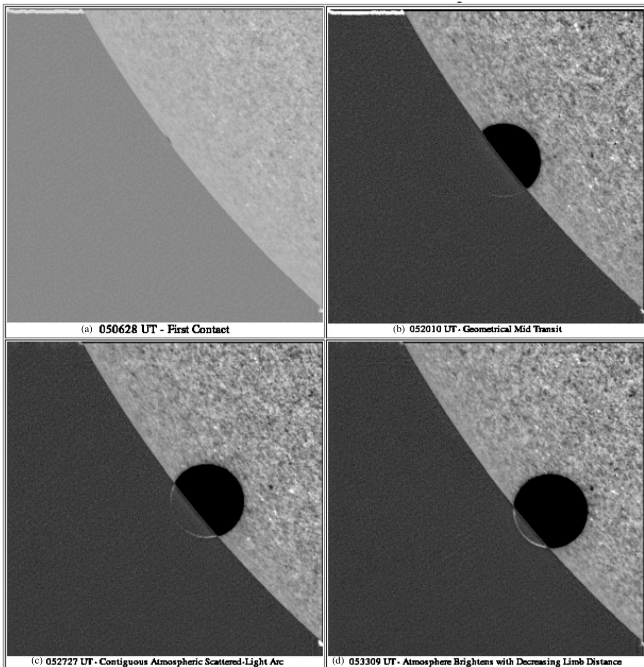
Figure 2. Ingress: (a) first contact (05:06:28 UT), a tiny black dot along the solar limb. (b) Geometrical mid limb transit (05:20:10 UT), with the appearance of a partial arc of sunlight refracted by the Cytherean atmosphere near the planet’s south pole. (c)–(d) The evolutionary appearance of the atmospheric arc (05:27:27 UT and 05:33:09 UT, respectively) is azimuthally asymmetric in brightness and increases in intensity with closing distance to the solar limb. All frames here, and in Figures 3–5, are oriented with north up and east to the left.
