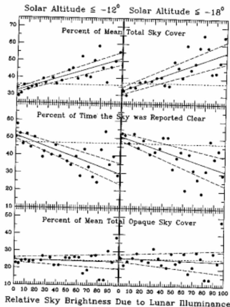
FIG. 4. The dependencies of the reported mean total sky cover, percentage of time the sky was reported clear, and percentage of reported mean opaque sky cover on the sky brightness due to moonlight during the austral polar winter, are shown in the top, middle and lower sets of figures, respectively. Results are plotted for times bounded by nautical (left column) and astronomical (right column) twilights. The significance of the solid and dashed lines are explained in the text.
