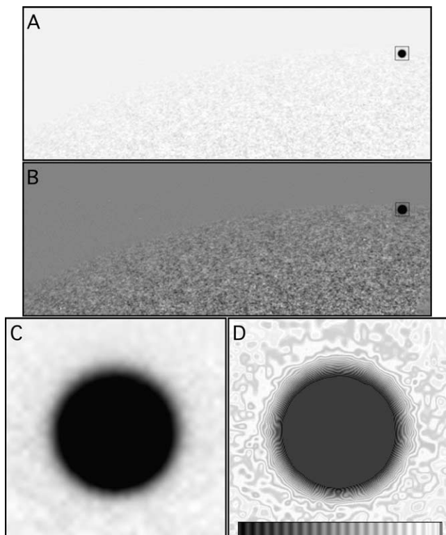
Fig. 8. The result of subtracting the PSF-broadened azimuthally averaged photospheric brightness profile from each image (A). The image below (B) is stretched to better show the mercurian disk and photospheric granulation. The images of the mercurian disk are enlarged in (C) and (D).
