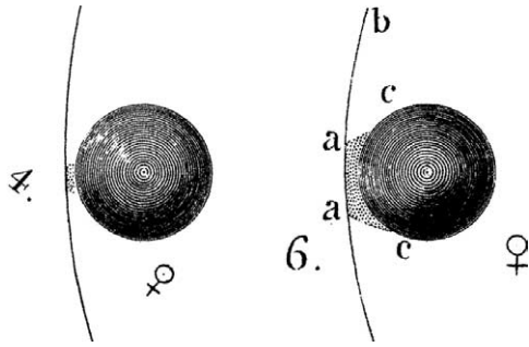
Fig. 1. Bergman (1761–1762) rendition of the Black Drop effect during the 1761 transit of Venus. Reprinted with permission from the Royal Society.
