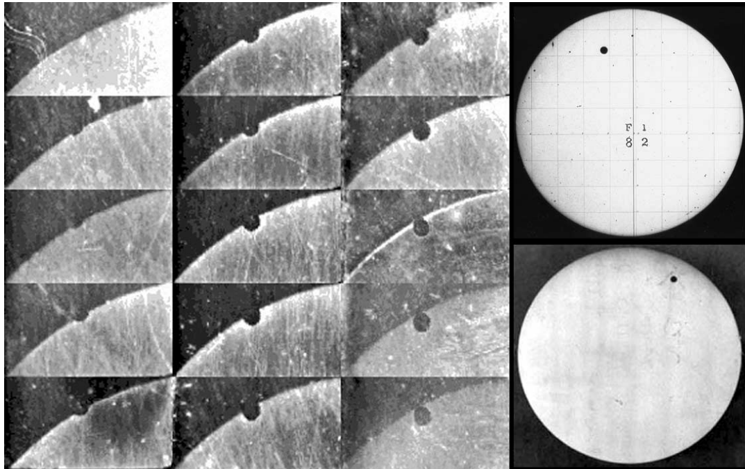
Fig. 3. Photographic images of the 19th century transits of Venus. (Left) Daguerreotypic time-resolved ingress sequence of the 1874 transit credited to Janssen using his “photographic revolver” ( http://web.inter.nl.net/users/anima/chronoph/index.htm ) (Janssen, 1873, 1876; Flammarion, 1875; Anonymous, 1875; Canales, 2002), though it may well be only a pre-transit test plate rather than an actual transit plate. (Right) The 1882 transit; one of eleven surviving images taken by the United States Naval Observatory (top, courtesy of USNO); photograph by Maria Mitchell and her students at Vassar College (bottom, reprinted with permission from Archives and Special Collections, Vassar College Libraries). South is up in both 1882 transit images.
