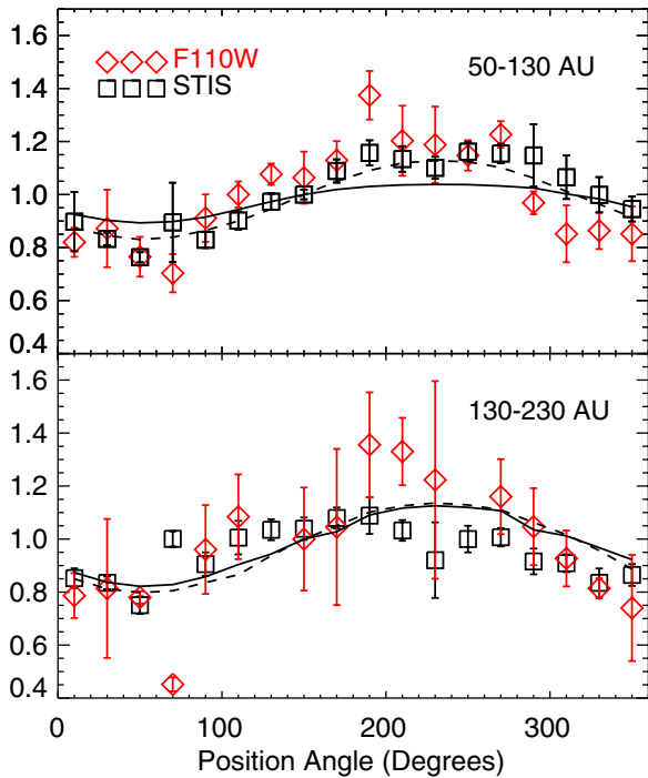
Figure 4. Azimuthal brightness profiles for the STIS and F110W images between 50–130 AU (top) and 130–230 AU (bottom). Each curve was normalized by the median surface brightness. In each panel, we compare the brightness asymmetry with that of our best-fitting model disk in Section 4.5 with inclinations of 7^\circ (solid line) and 7^\circ with a g parameter of 0.5 (dashed line). Both models assume that the P.A. of the disk is aligned with the side of the disk closest to the observer. For the isotropic model, the disk P.A. is 53^\circ 6' , while the forward scattering model has a P.A. of 233^\circ 6' .
